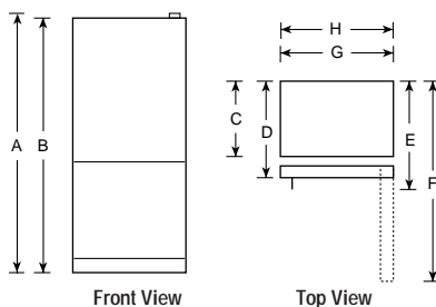
Bottom-Mount Refrigerator
