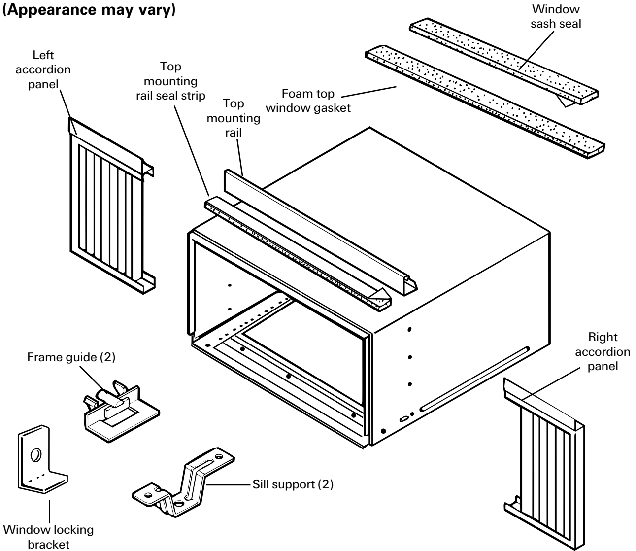
Type B (3)
