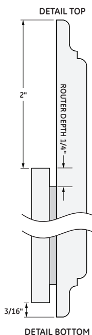
DETAIL TOP DETAIL BOTTOM
