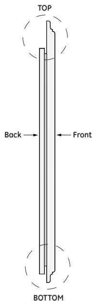
3/4" PANEL SIDE VIEW (AFTER ROUTING)
