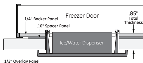
1/2" OVERLAY PANEL DISPENSER TRIM
