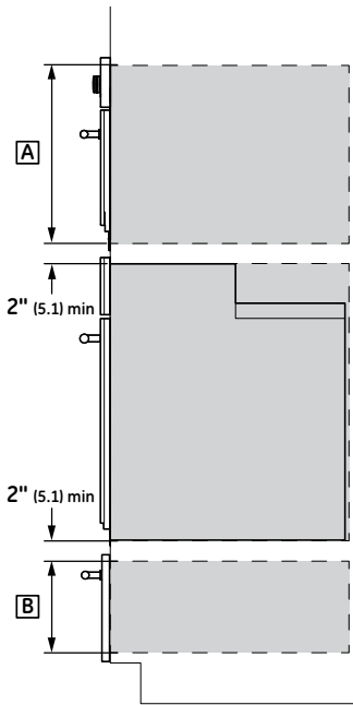
STANDARD INSTALLATION SIDE VIEW
