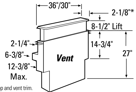
Models JVB67A/37A
