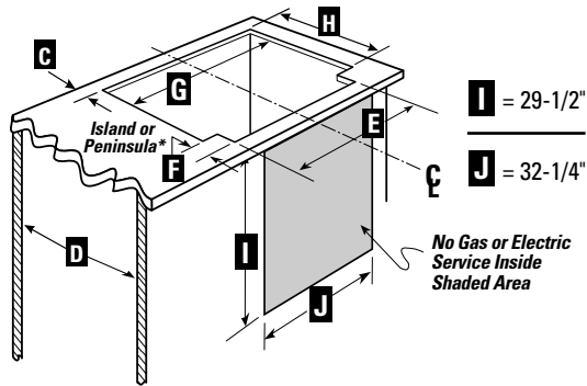
Fig. 2 Cutout for models JVB96SA/93SA only
