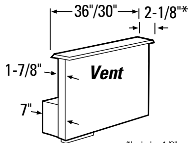
Models JVB96SA/93SA
