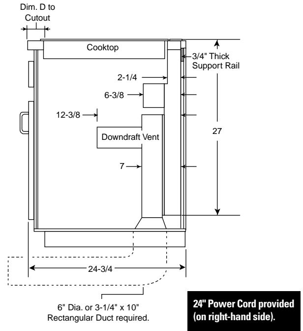
Fig. 4 Venting Island to Outside Wall
