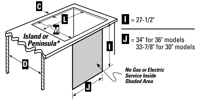
Fig. 3 Cutout for model JVB67A/37A only
