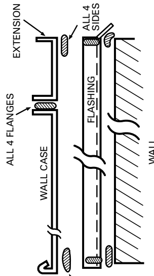
SECTION A-A BASEPAIN/FLANGE DESIGN SHOWING SEALANT LOCATIONS.
