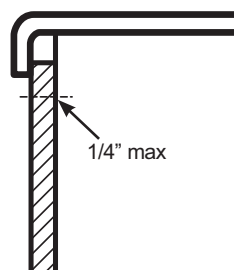
Panels 1/4" thick or less
