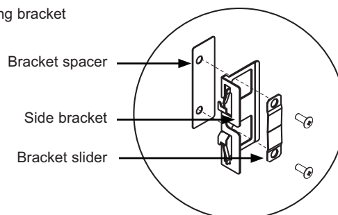
Left side installation when facing rear of the door panel
