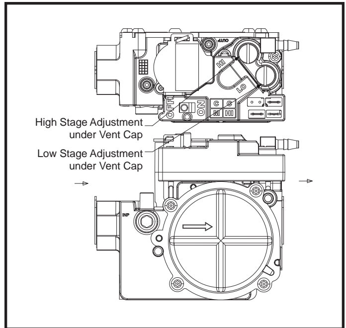
Figure 2. Two-Stage Gas Valve
