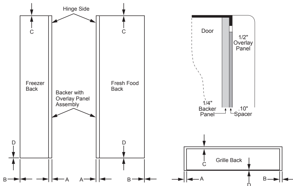
PANEL DIMENSIONS
