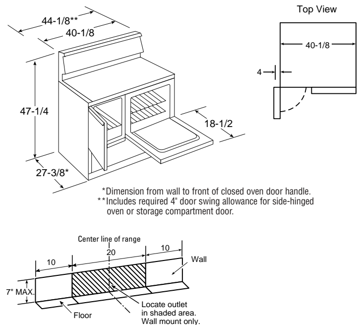
40" Range Dimensions and Installation Information (in inches)
