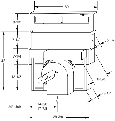
Model JVB37
