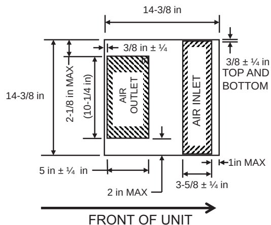
Low Profile Models (PLCS/PLHS) TOP-DOWN VIEW
