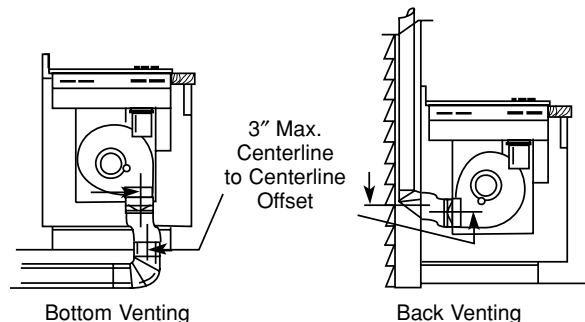
Bottom Venting
