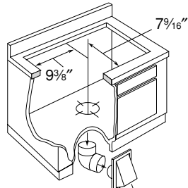
Downward Venting
