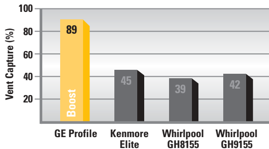
The GE 315-CFM venting system at “boost” settings, compared to competitors’ “high” setting.
