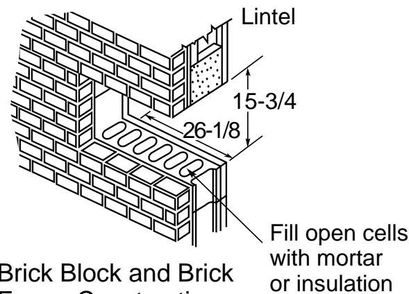
Frame Construction
