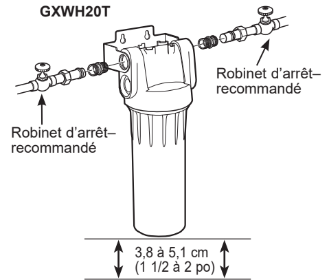
GXWH20T
