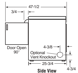
Dryer Dimensions (in inches)
