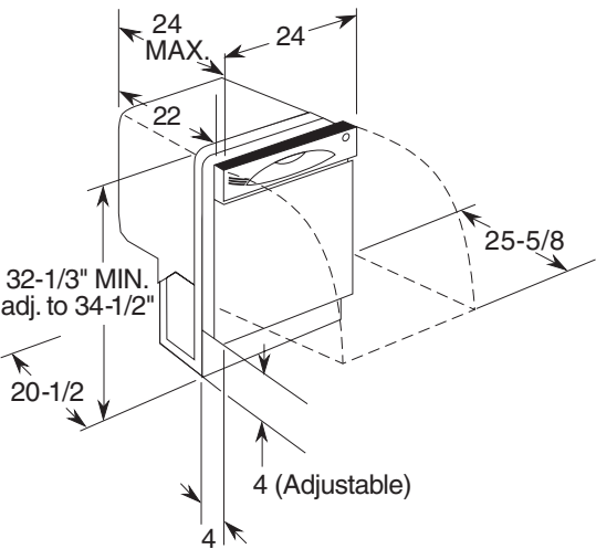
Dishwasher Dimensions (in inches)
