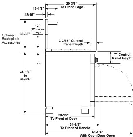
SIDE VIEW WITH BACKSLASH
