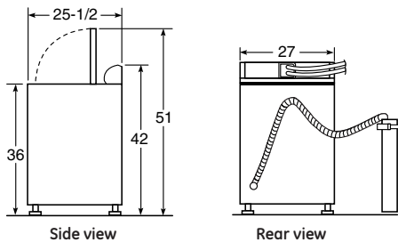
Washer dimensions (in inches)
