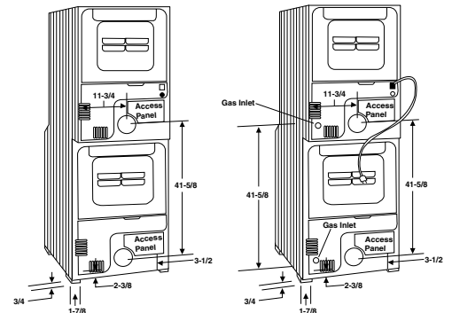
DDC4400S Back view
