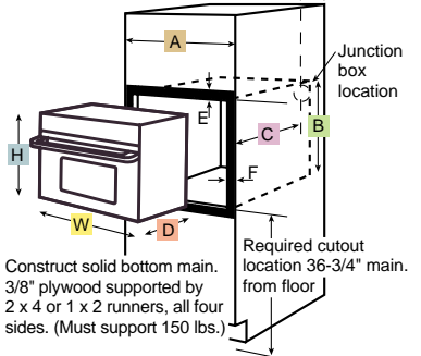
Advantium Wall Oven
