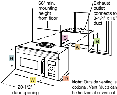
Advantium® Above-The-Cooktop Oven
