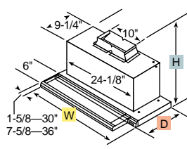
Slide-Out Hood
