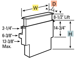
Telescopic Downdraft System
