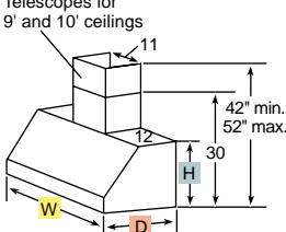
Designer Hood
