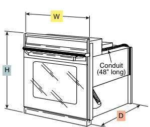
Single Wall Oven
