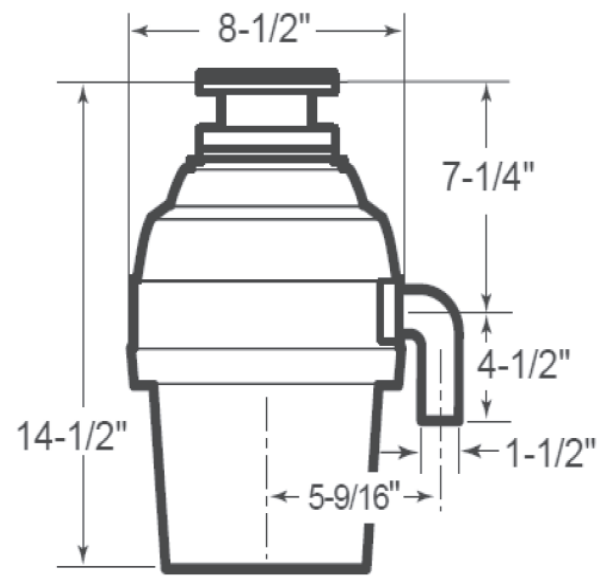
Disposall® Food Waste Disposer Dimensions (in inches)
