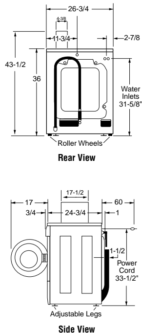
Washer Dimensions (in inches)
