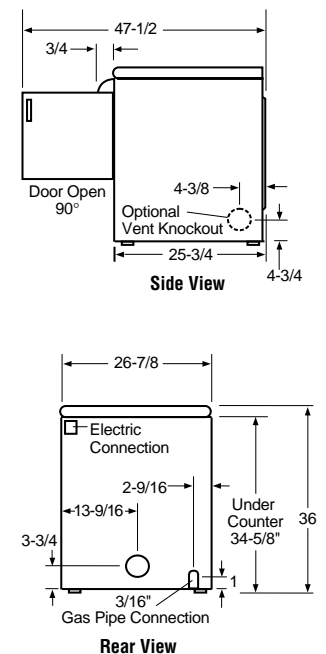
Dryer Dimensions (in inches)
