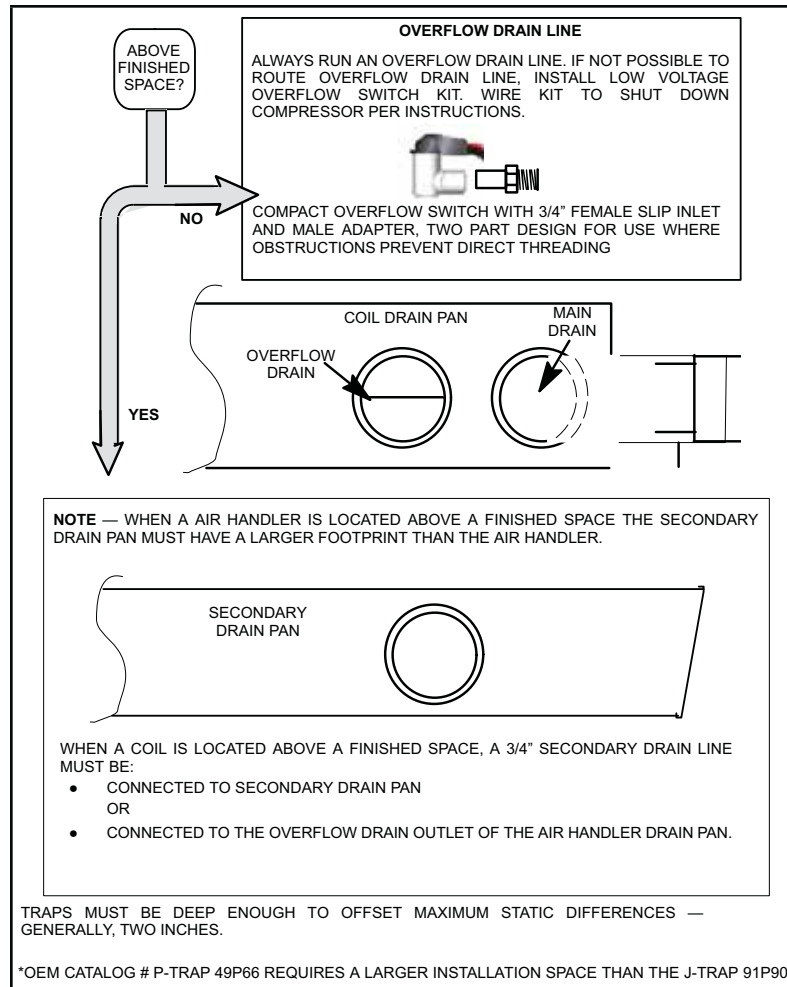
FIGURE 8. Typical Main and Overflow Drain Installations
