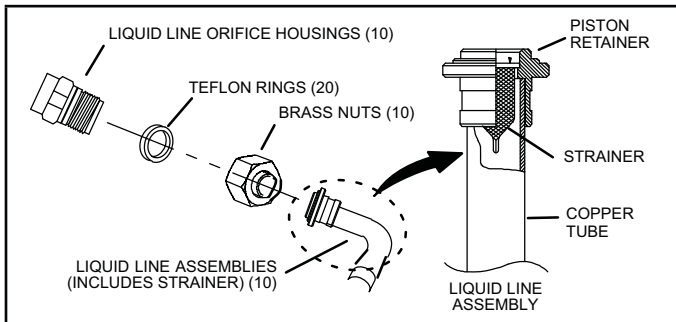
FIGURE 1. 69J46 Kit Components
