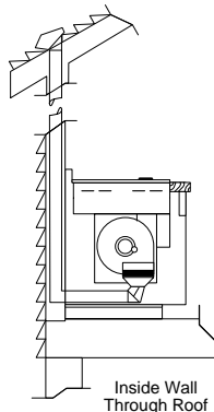
Inside Wall Through Roof
