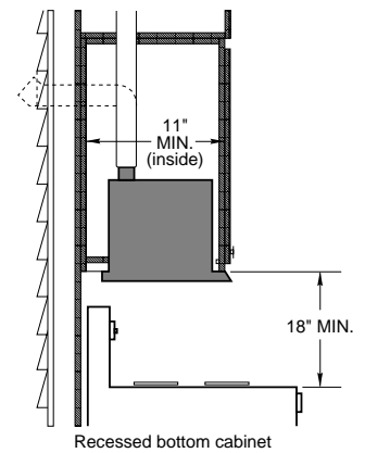
Recessed bottom cabinet
