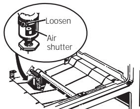
Bake Burner
