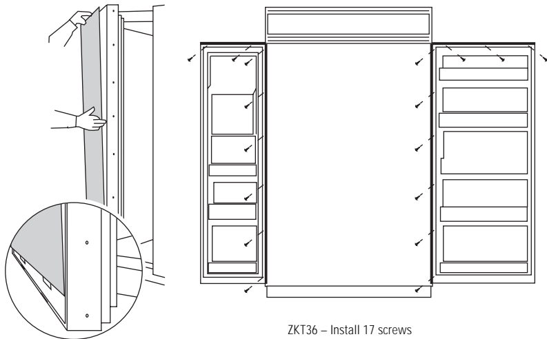
ZKT36 - Install 17 screws
